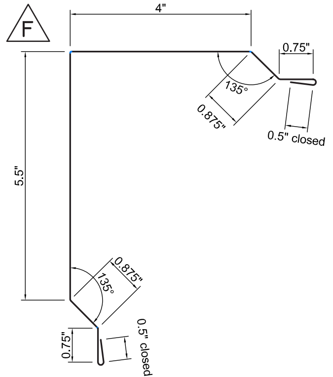
PF03 POST FRAME GABLE TRIM
