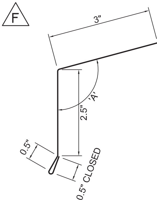
PF31 EAVE EDGE 4:12 PITCH STANDARD UNLESS SPECIFIED OTHERWISE
