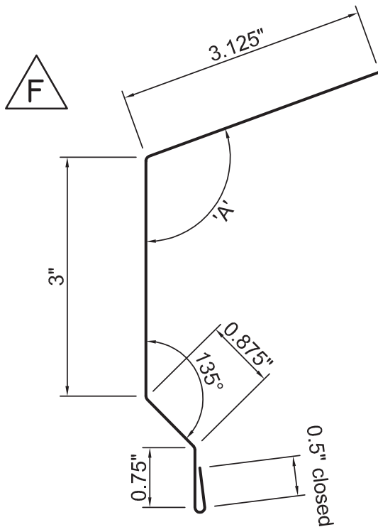
PF09 POST FRAME EAVE TRIM 4:12 PITCH STANDARD UNLESS SPECIFIED OTHERWISE
